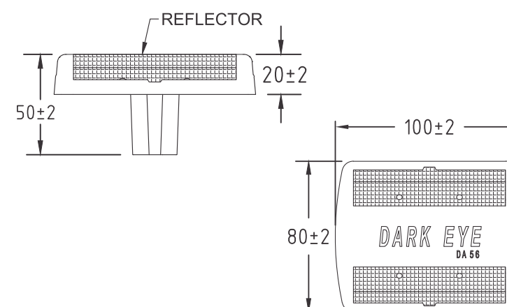
MODEL NO. : DA 56 TWO WAY REFLECTIVE Dimensions 100 x 80 x 20 mm Aluminium Alloy body Reflective Panel - Amber, Red or White Weight : 185 Grams
