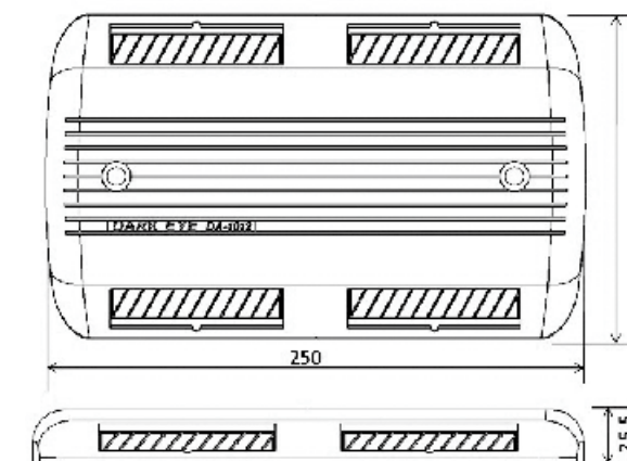
MODEL NO. : DA 1012 Weight : 510 Grams
