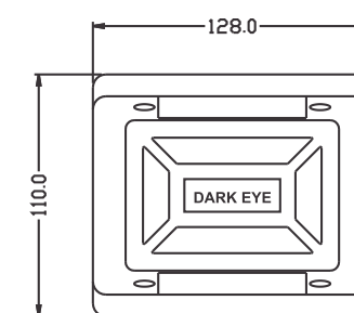
MODEL NO. : DA 971 TWO WAY REFLECTIVE Dimensions 110 x 128 x 30 mm Aluminium Alloy body Reflective Panel- Amber, Red or White Weight : 530 Grams
