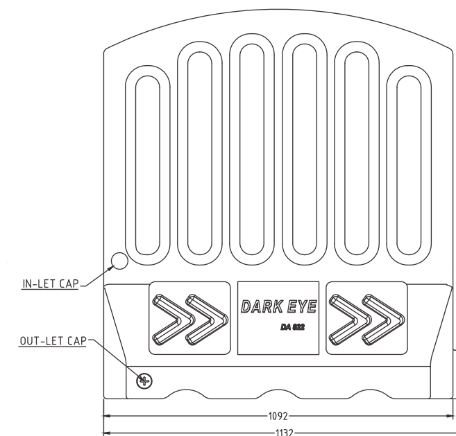
Model - DA 822 Weight : 8500 GM HEIGHT : 1220 MM MATERIAL : HDPE
